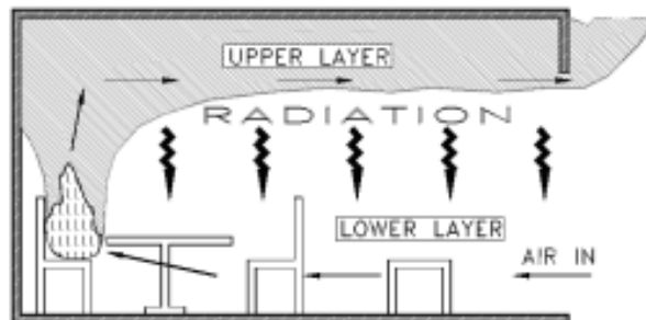
Figure 1 – Room Fire Dynamics
